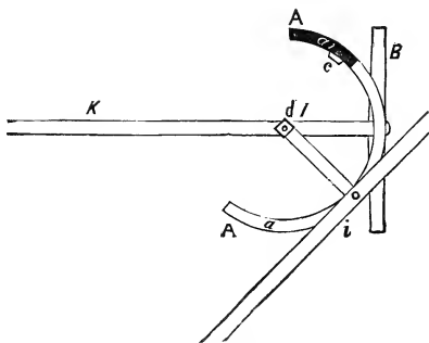
ANOTHER HAUSSKNECHT COUPLING.
